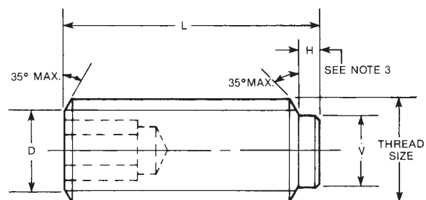
DOG POINT
