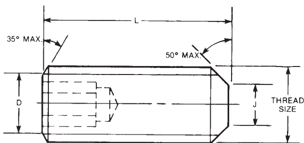
FLAT POINT
