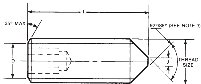
CONE POINT
