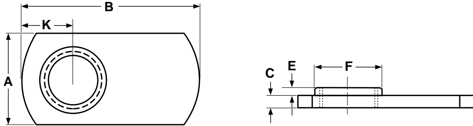
TAB WELD NUTS, OFFSET HOLE WITHOUT PROJECTIONS
